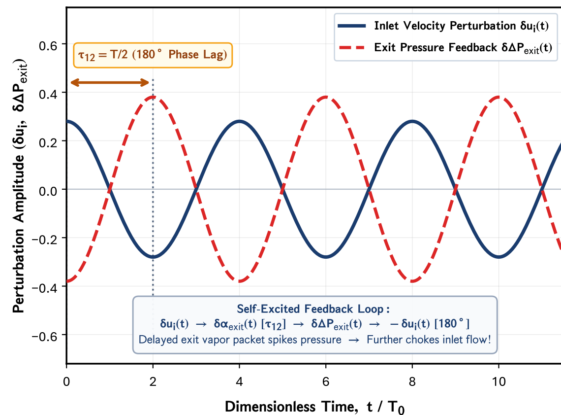
(e) Dynamic Density-Wave Transit Delay \tau_{12} & Feedback
