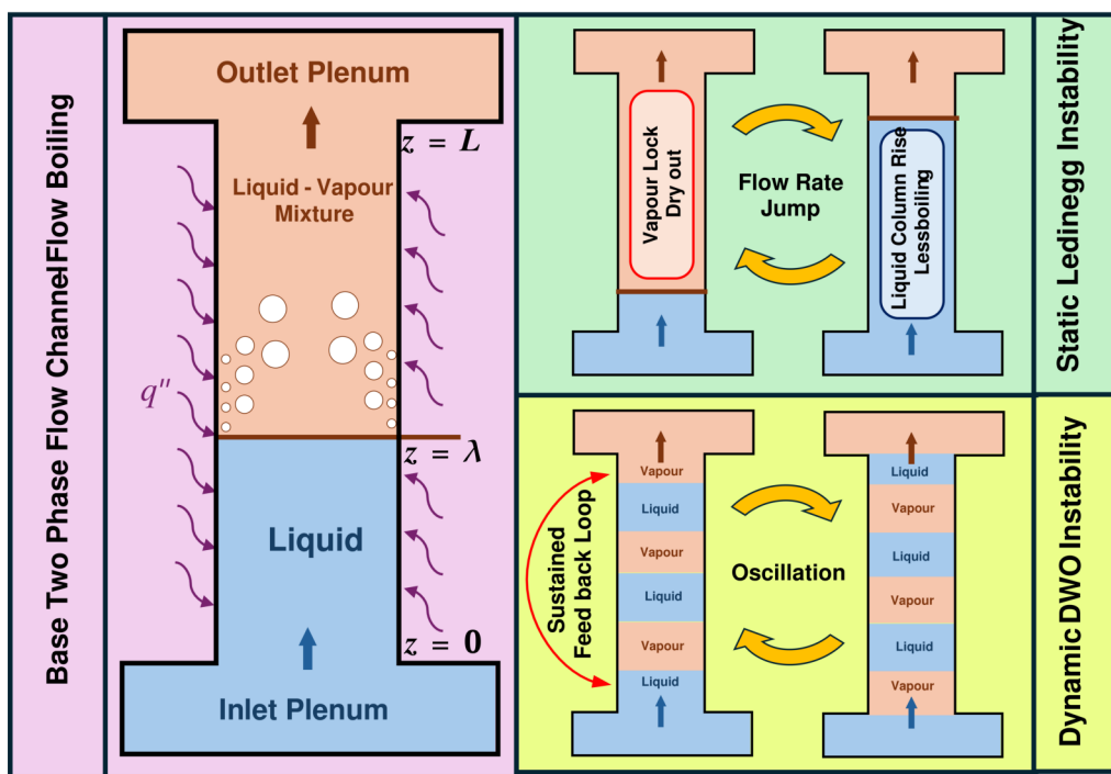
(a) Boiling Physics &amp; Instability Mechanisms
