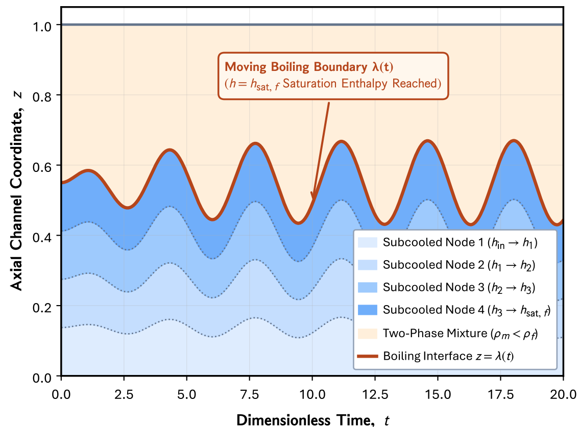
(b) Multi-Node Enthalpy Field Evolution
