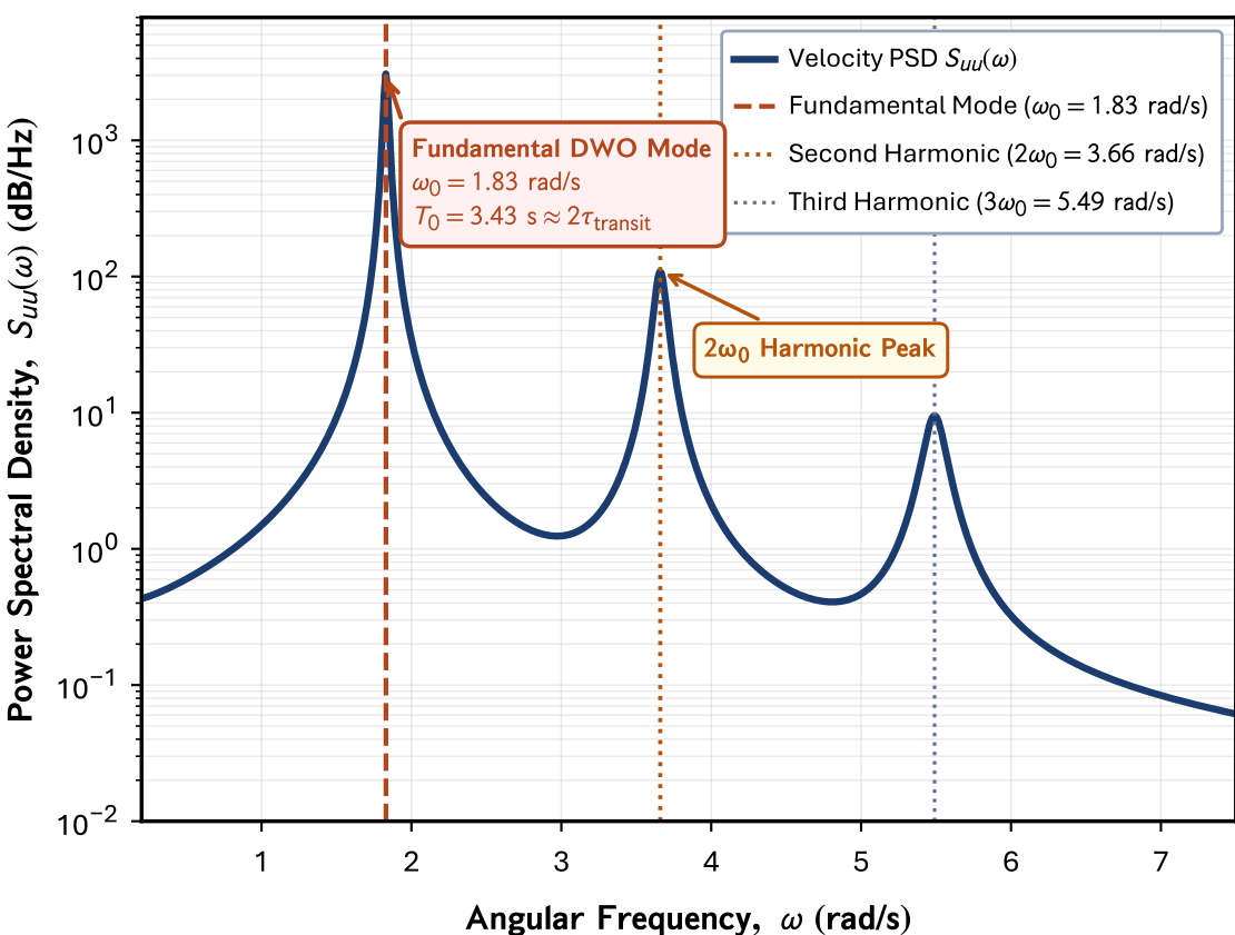
(c) Spectral Frequency Analysis (FFT)
