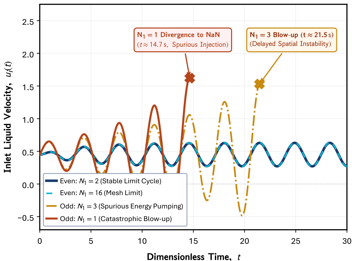
(a) The Odd-Node Energy Pumping Pathology
