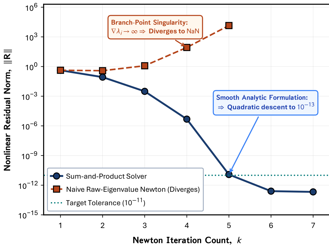
(f) 2D Newton Sum-and-Product Solver Convergence
