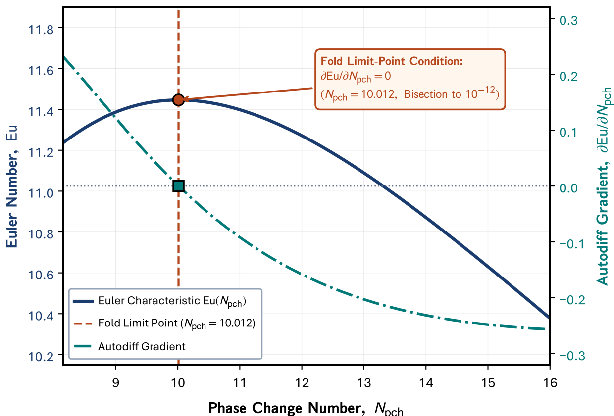
(e) Autodiff Fold Continuation ( \partial Eu / \partial N_{pch} = 0 )
