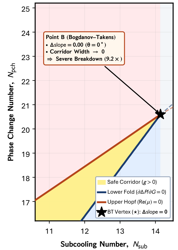
(b 2 ) Point B : Tangential Cusp ( \Delta\text{slope} = 0.00 )
