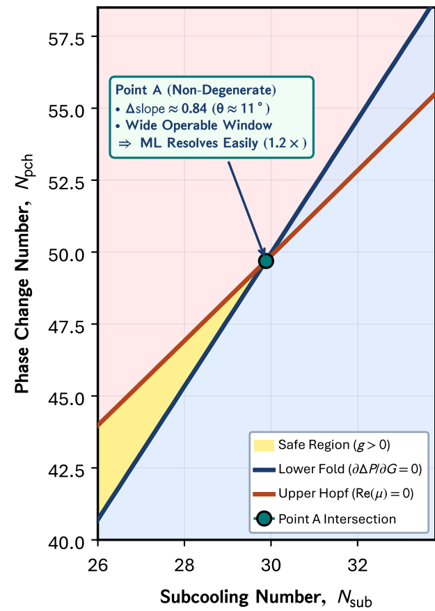
(b 1 ) Point A : Transversal ( \Delta\text{slope} \approx 0.84 )
