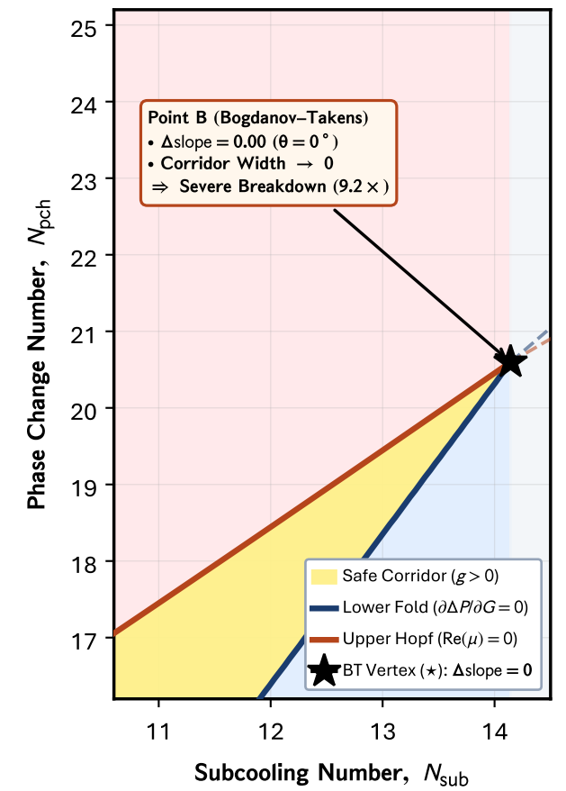
(b 2 ) Point B : Tangential Cusp ( \Delta\text{slope} = 0.00 )
