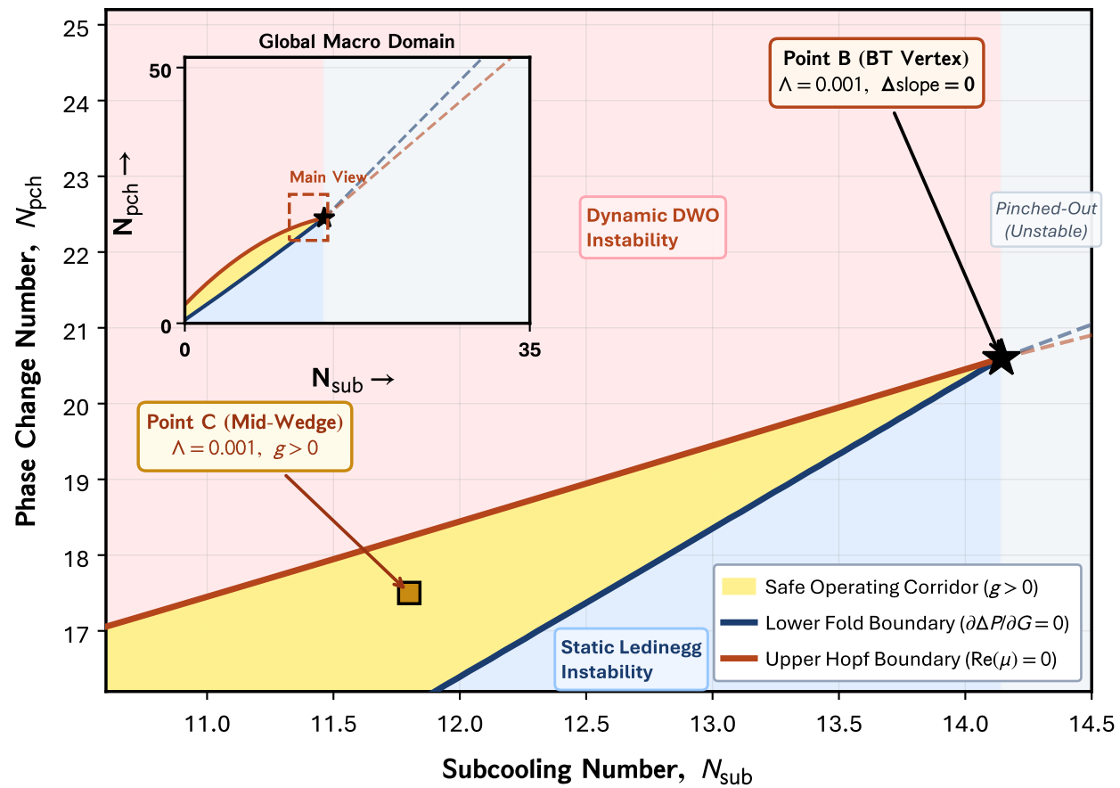
(a) Geometry of the Knife-Edge Stability Wedge
