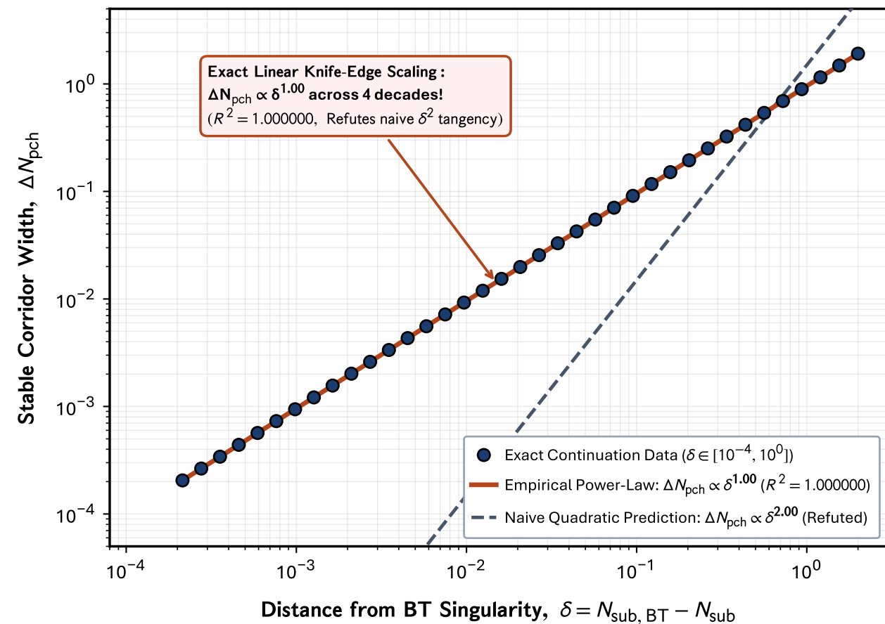
(c) Multi-Decade Stable-Window Power-Law Scaling
