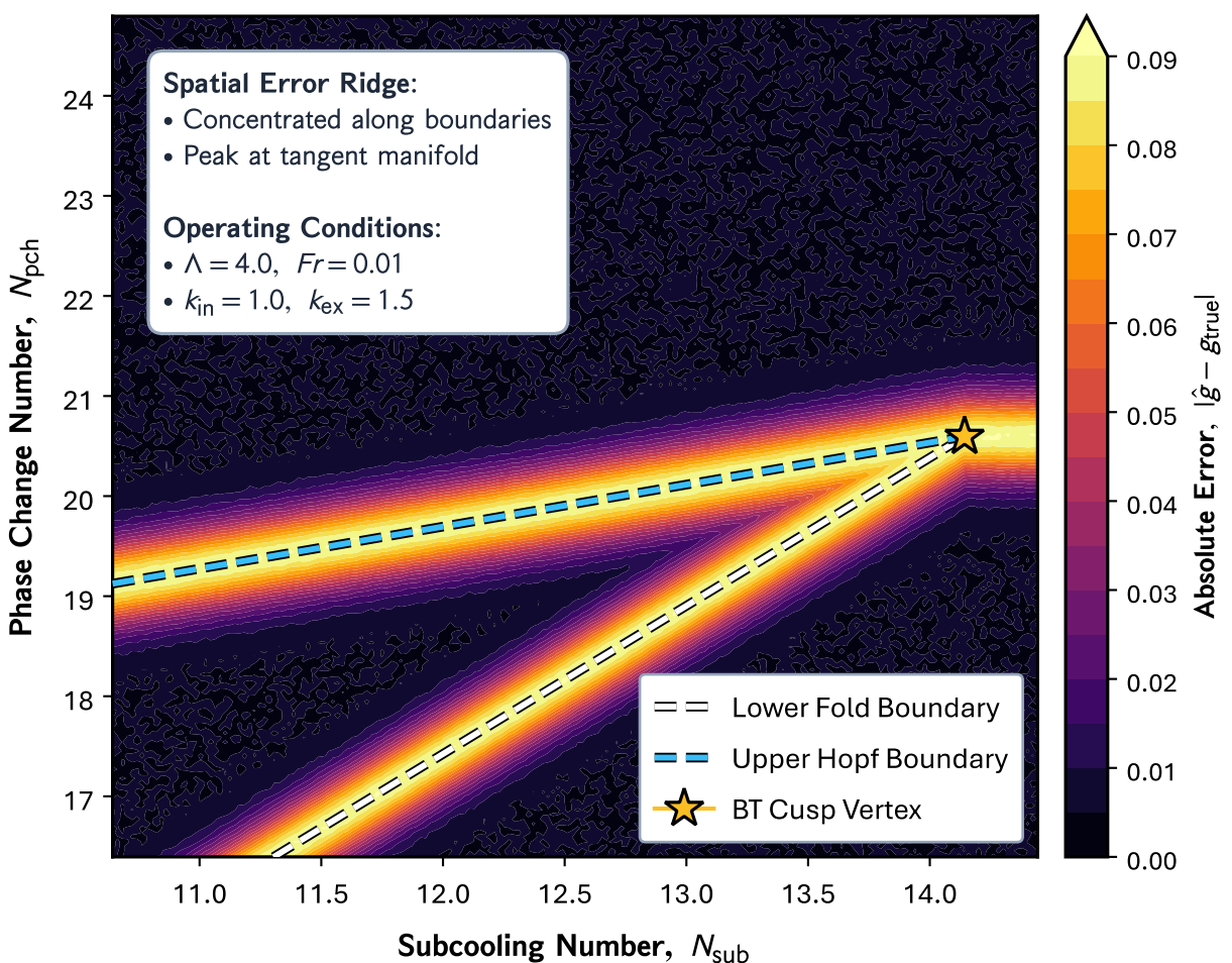
(e) 2D Spatial Error Field |\hat{g}(x) - g_{true}(x)| Near BT Cusp
