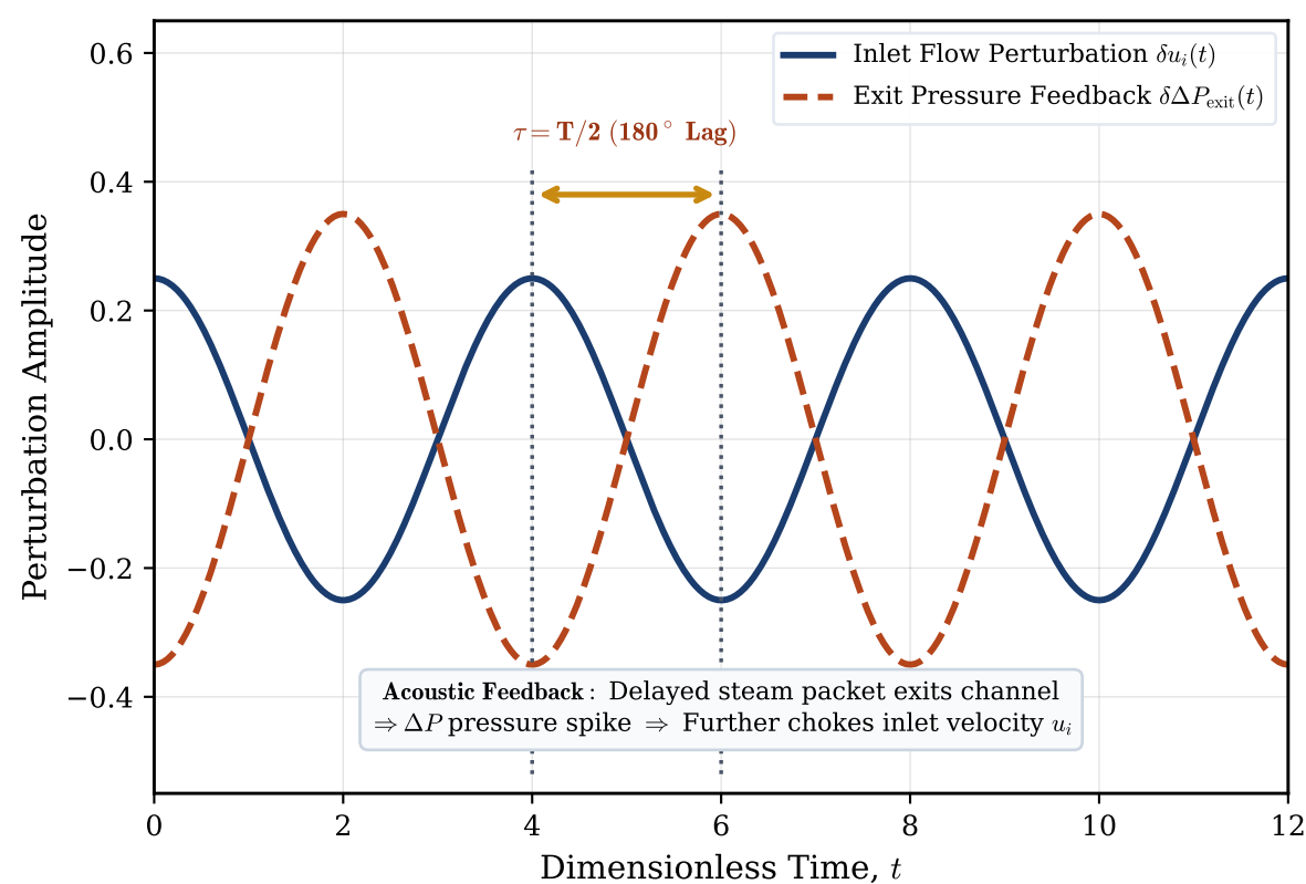
(e) Dynamic Density-Wave Transit Delay \tau
