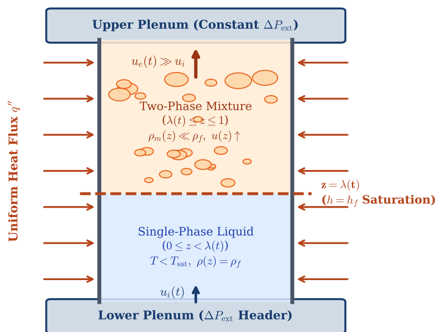
(a) Physical Zonation & Moving Boundary \lambda(t)
