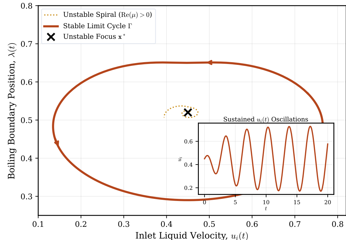
(f) Supercritical Hopf Limit-Cycle Orbit
