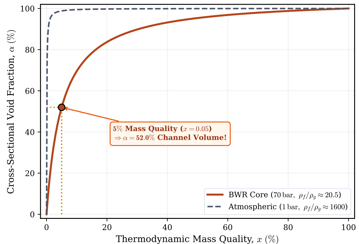
(b) Thermodynamic Void Non-Linearity
