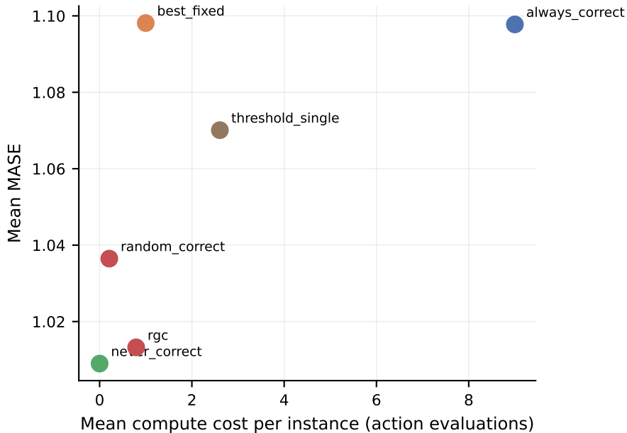
Accuracy vs. compute: is adaptivity cheaper?
