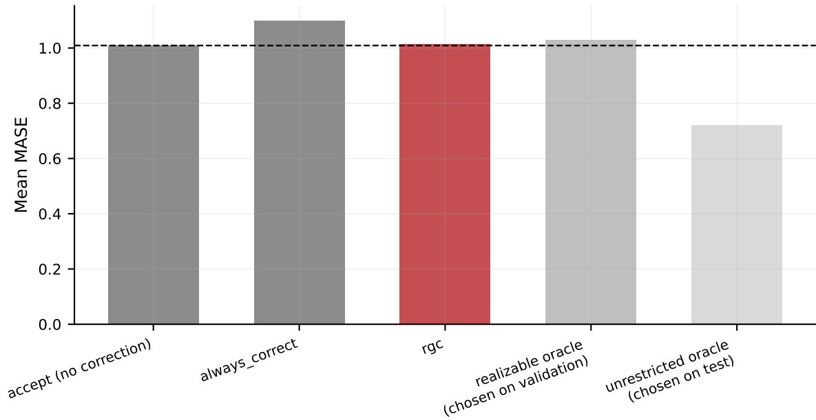
Achievable vs. apparent correction headroom
