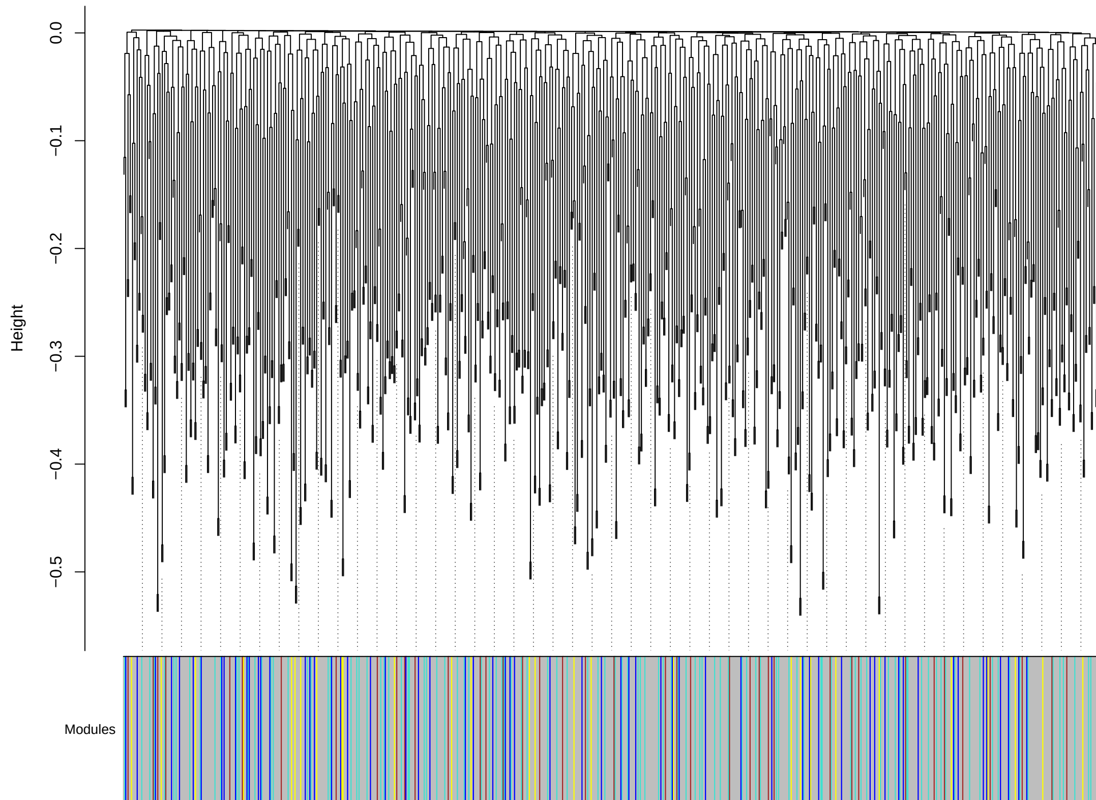
Gene Co-expression Network Dendrogram (Fast Rebuild)
