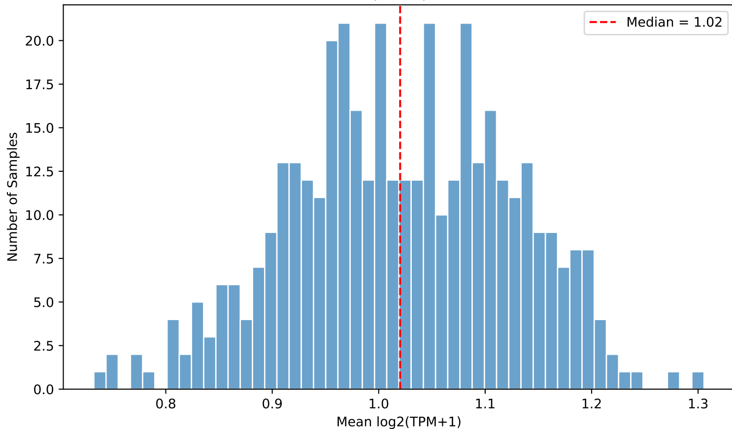
GTEx Stomach: Sample Expression Distribution
