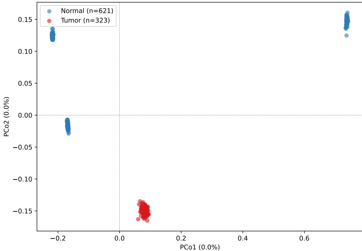
Beta Diversity: Bray-Curtis PCoA (DDBJ PRJDB20660, 944 samples)
