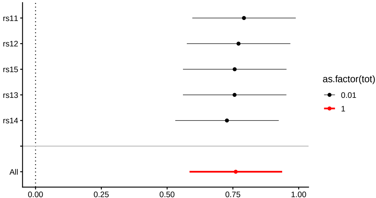
MR leave-one-out sensitivity analysis for 'H. pylori IgG seropositivity' on 'Stomach cancer'
