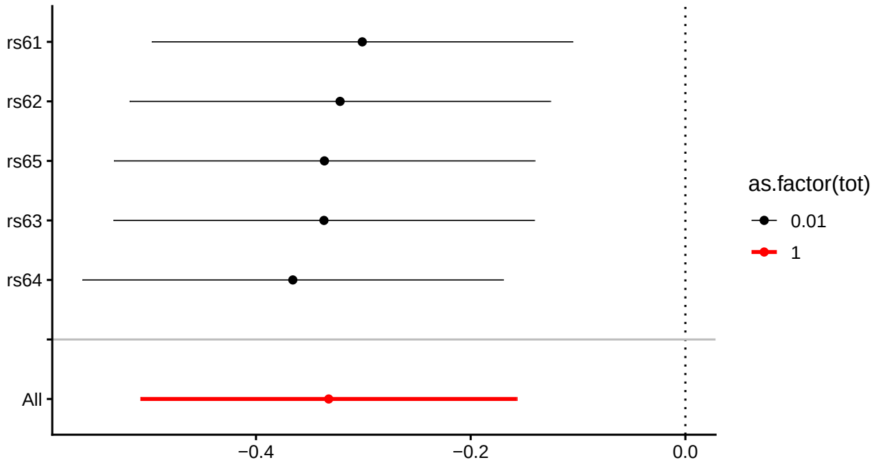
MR leave-one-out sensitivity analysis for 'genus Lactobacillus (protective)' on 'Stomach cancer'
