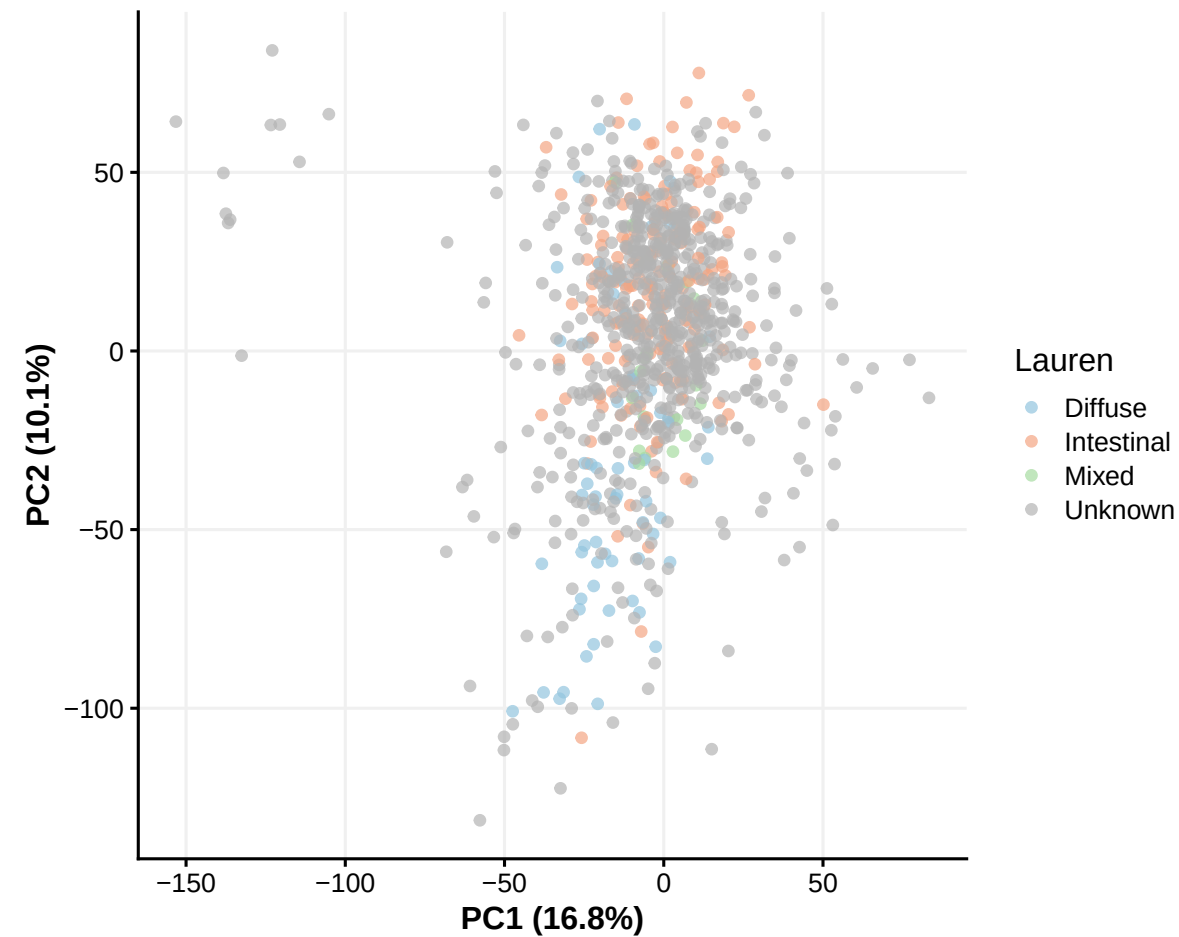
Combined Tumors ... Lauren Subtype
