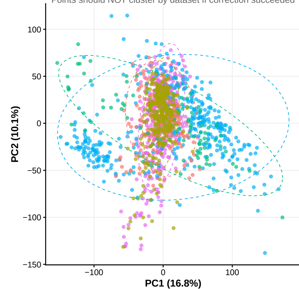
Combined Cohort ... Batch Check (post-ComBat)
