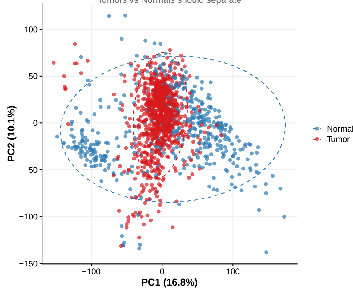
Combined Cohort ... Biological Signal
