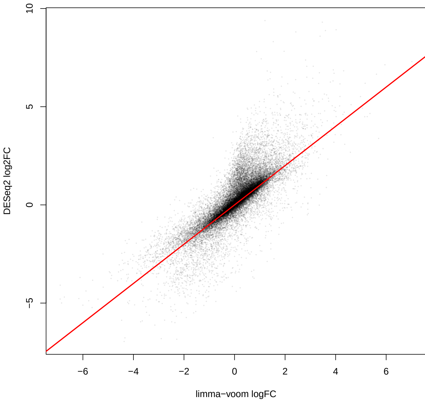
DEG Comparison (r=0.820, J=0.208)
