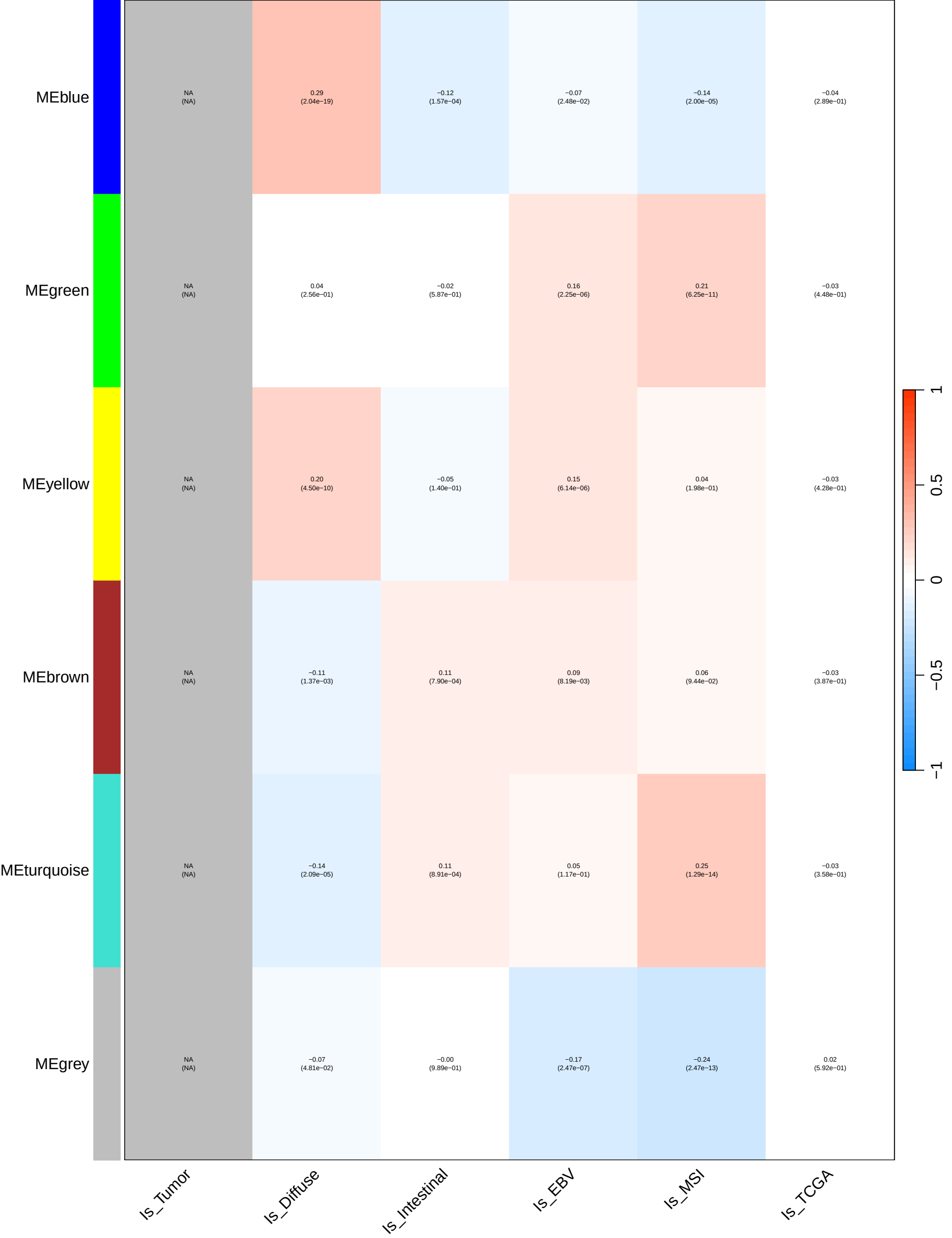
Module...Trait Correlation (Pearson r, BH-corrected p)
