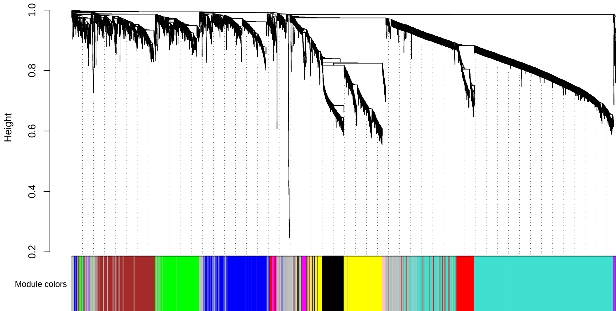
Gene dendrogram and module colors (TCGA-STAD, top 5000 MAD)
