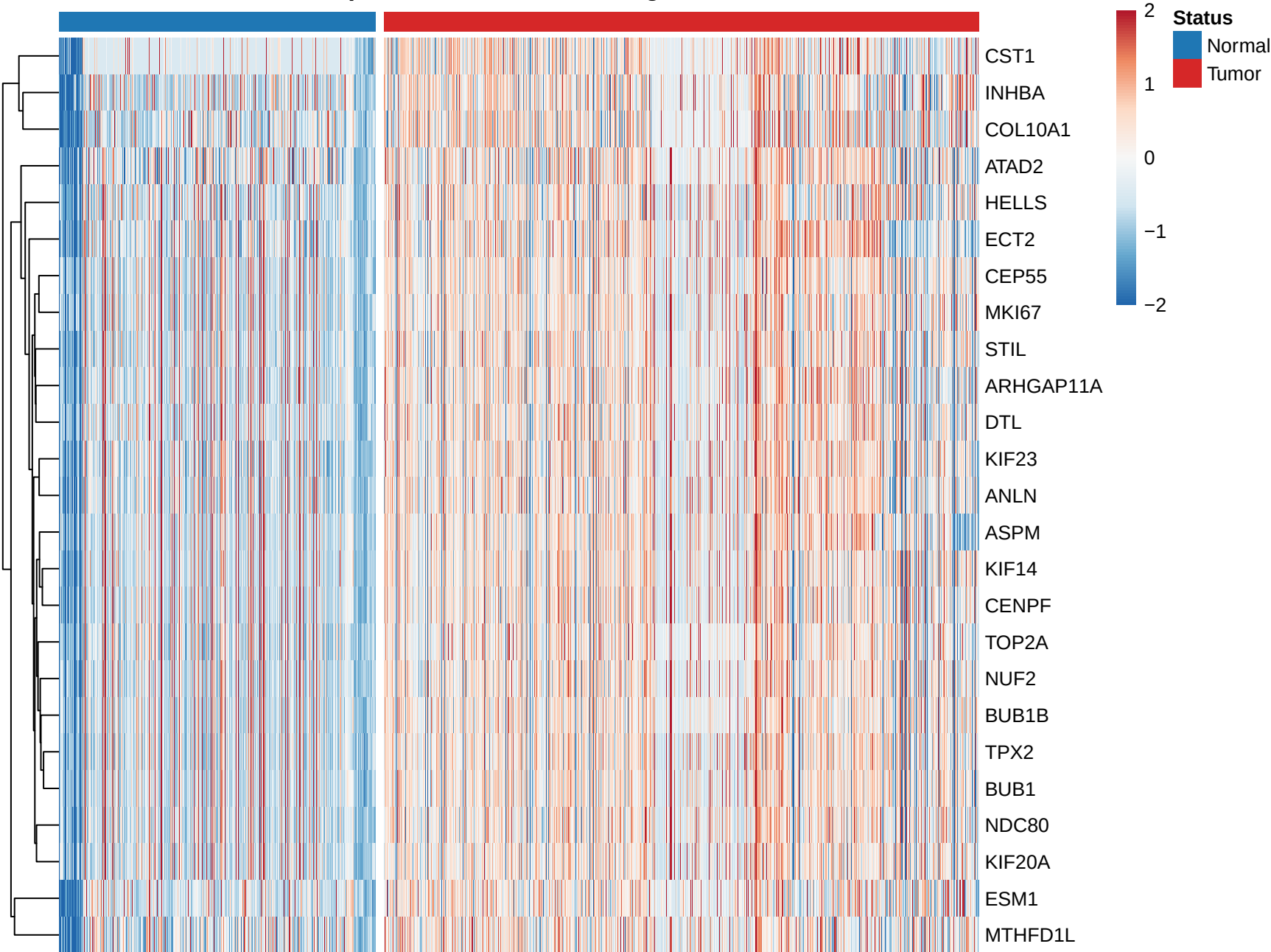
Top 25 tumour-vs-normal genes
