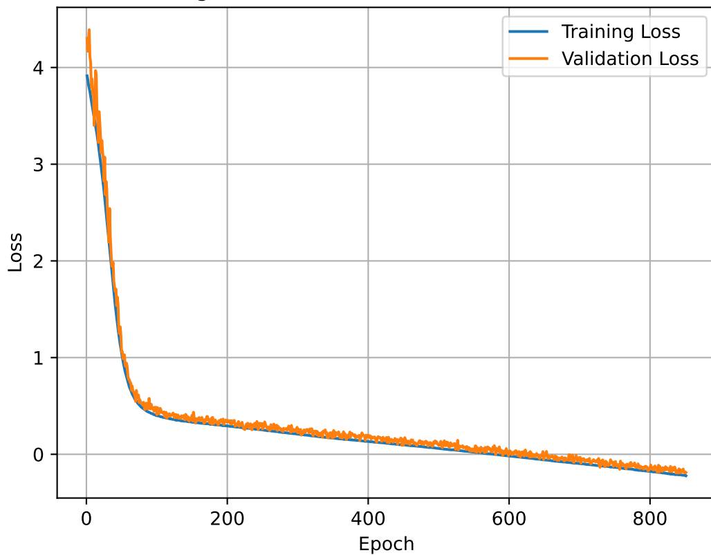
Training and Validation Losses for SMNR 20.0dB
