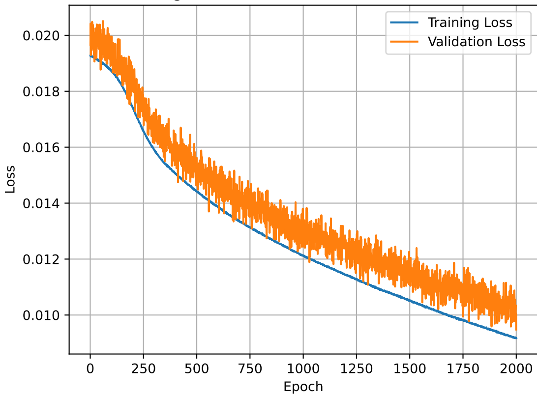
Training and Validation Losses for SMNR 5.0dB
