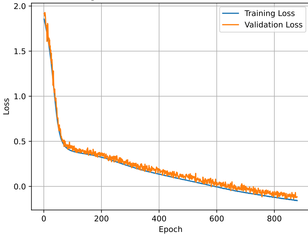
Training and Validation Losses for SMNR 10.0dB
