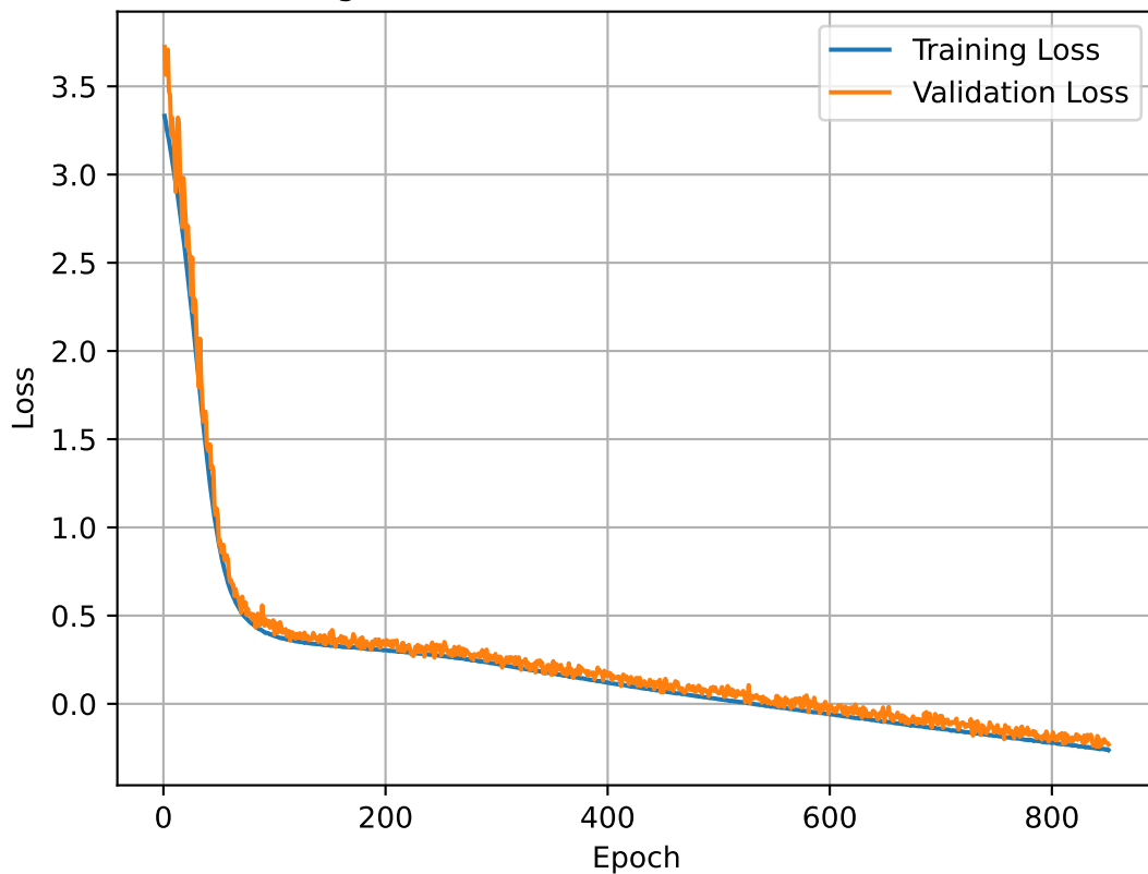
Training and Validation Losses for SMNR 20.0dB
