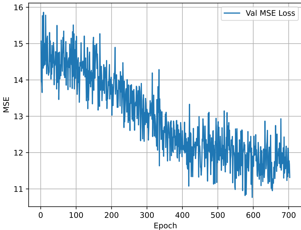
Validation MSE Losses for SMNR -5.0dB
