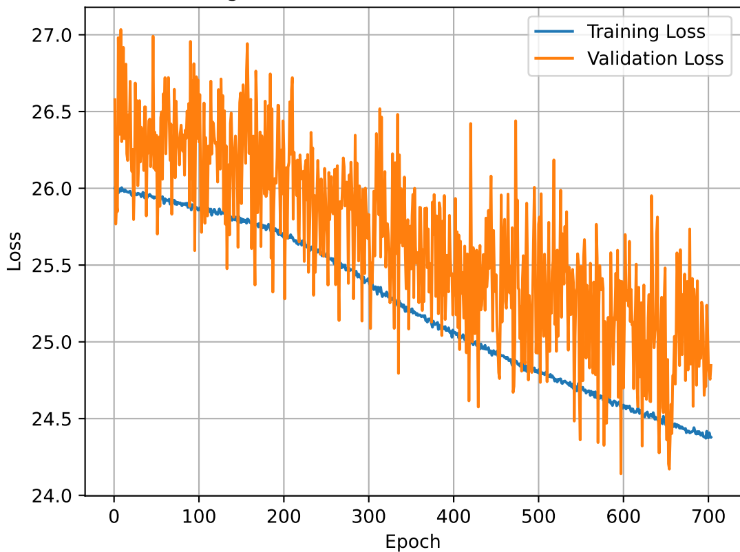
Training and Validation Losses for SMNR -5.0dB
