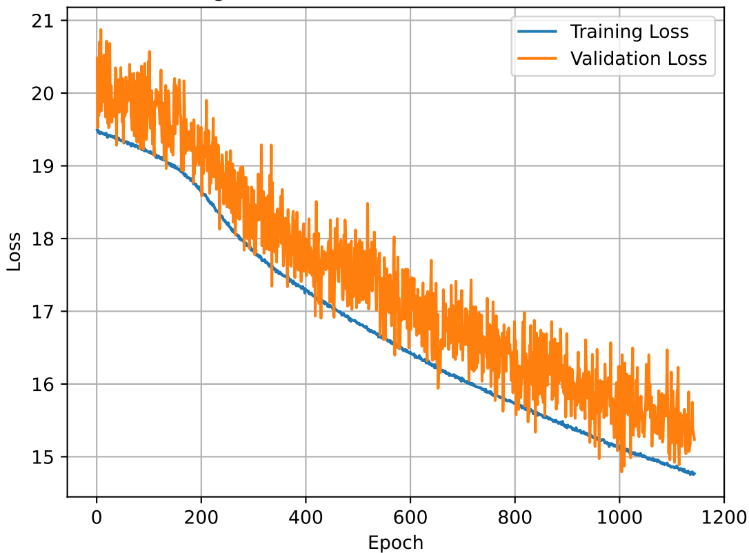
Training and Validation Losses for SMNR 0.0dB
