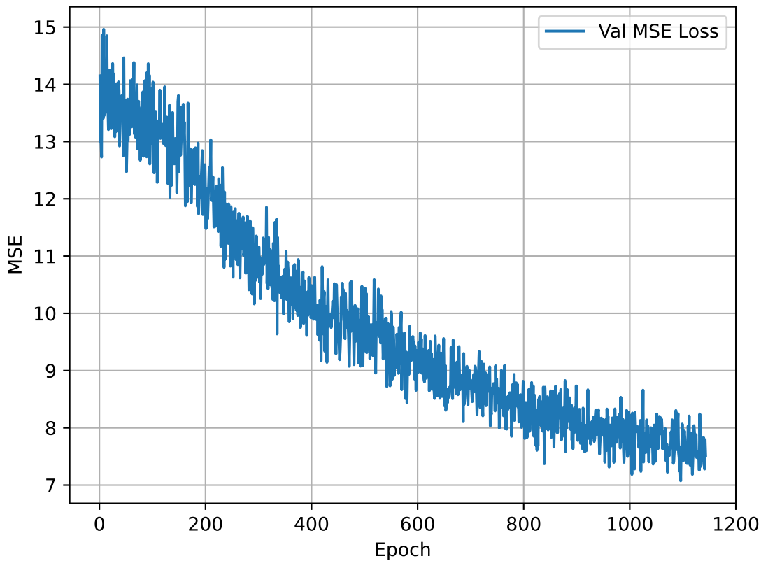
Validation MSE Losses for SMNR 0.0dB
