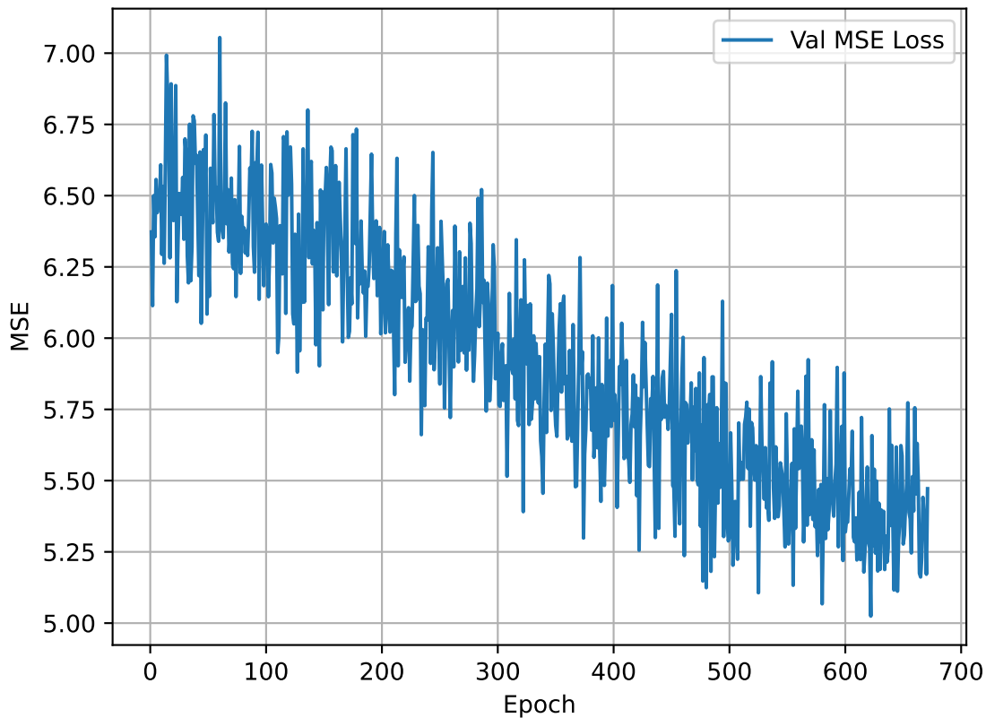
Validation MSE Losses for SMNR -5.0dB
