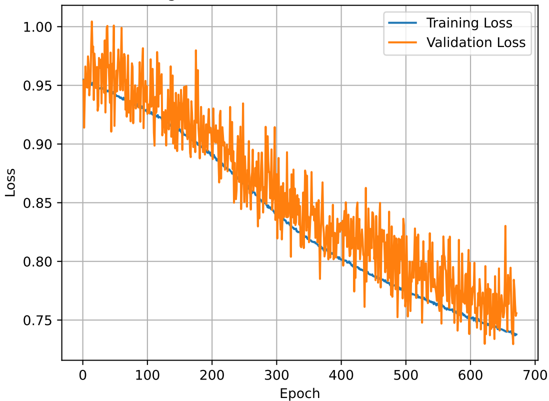
Training and Validation Losses for SMNR 0.0dB
