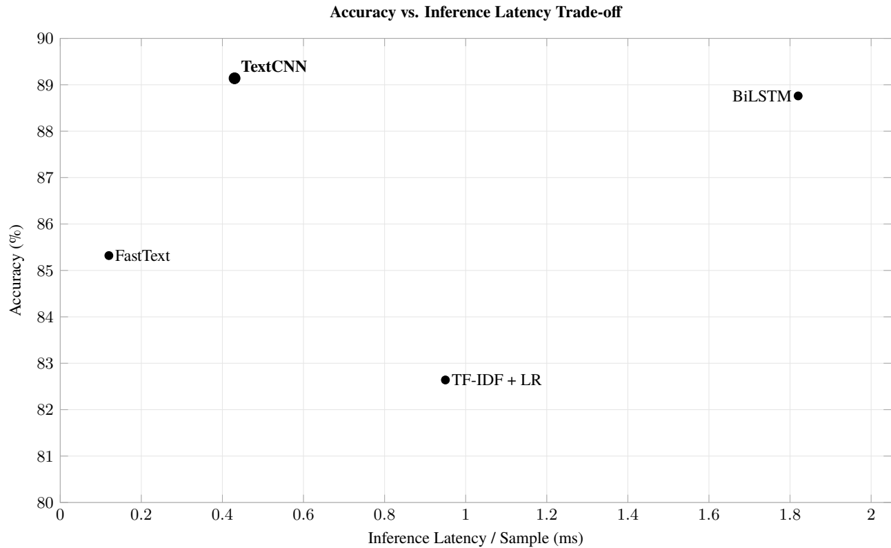
Figure 1: Accuracy versus inference latency for the evaluated models. The multi-scale 1D TextCNN provides the best overall trade-off, achieving 89.14% accuracy with an inference latency of 0.43 ms per sample.
