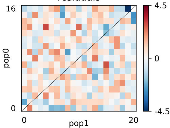
residuals
