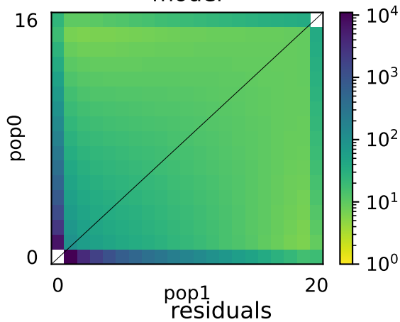
model
