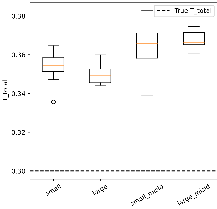
Total Divergence Time: T_{\text{WGD}} + T_{\text{dip}}
