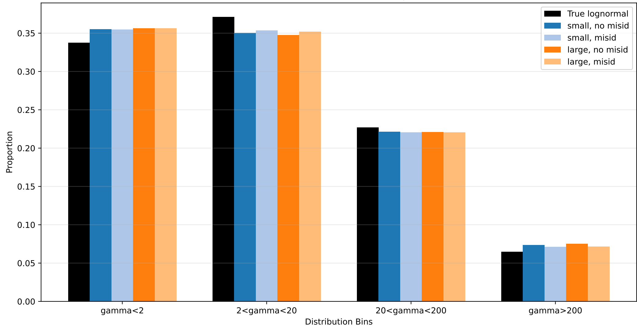
Discretized DFE Distribution Comparison
