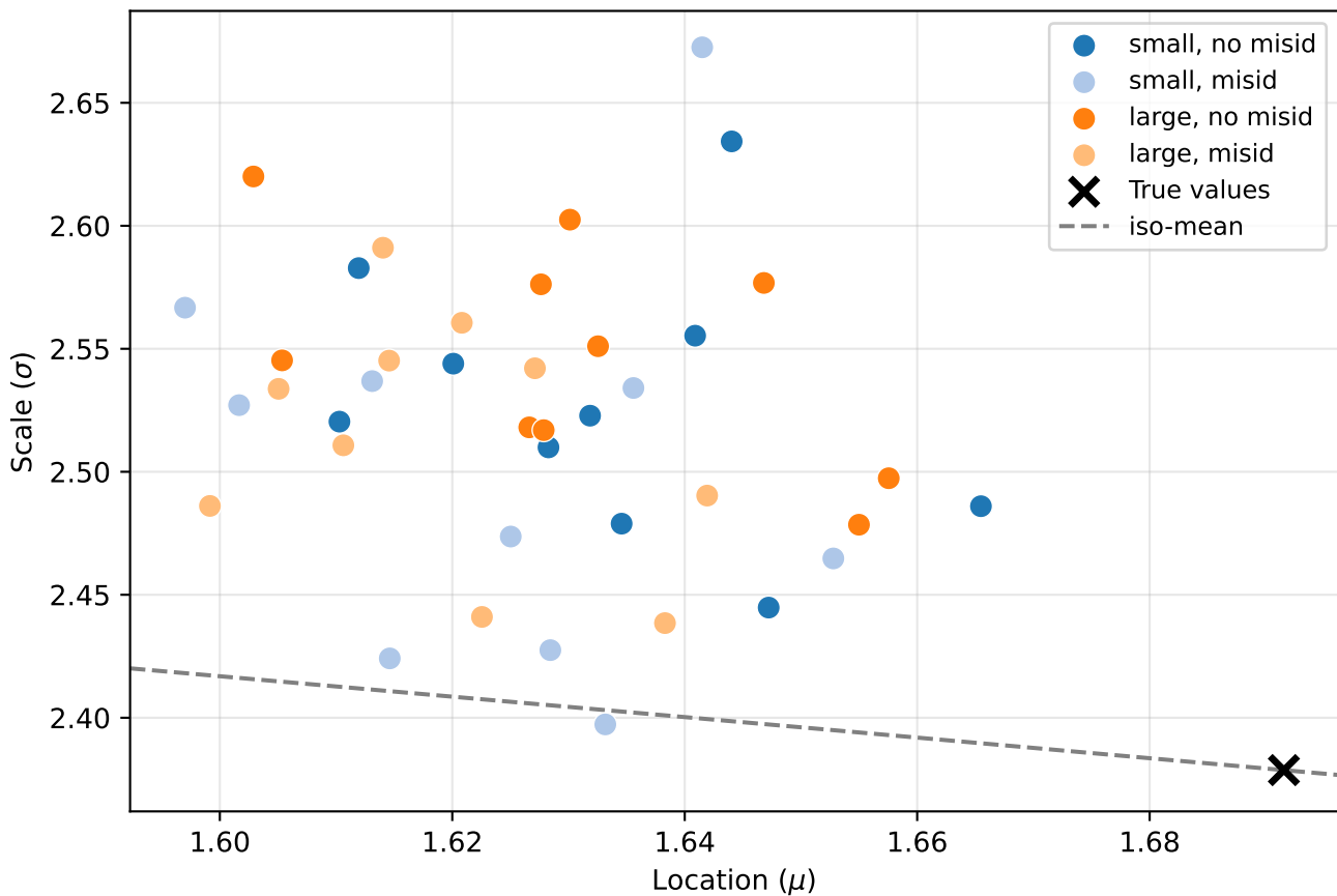
DFE Inference: Location & Scale
