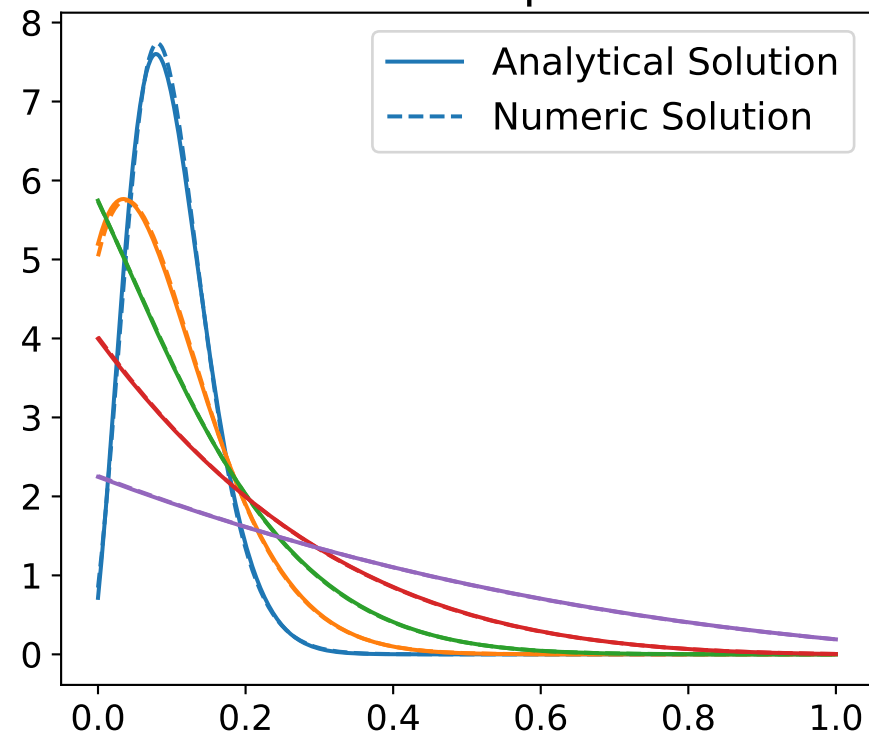
Autohexaploid
