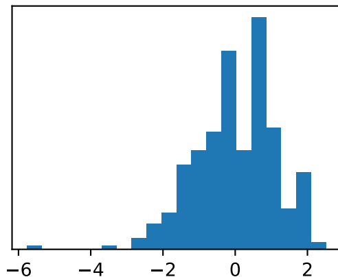
residuals
