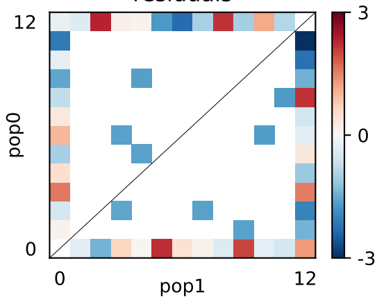
residuals
