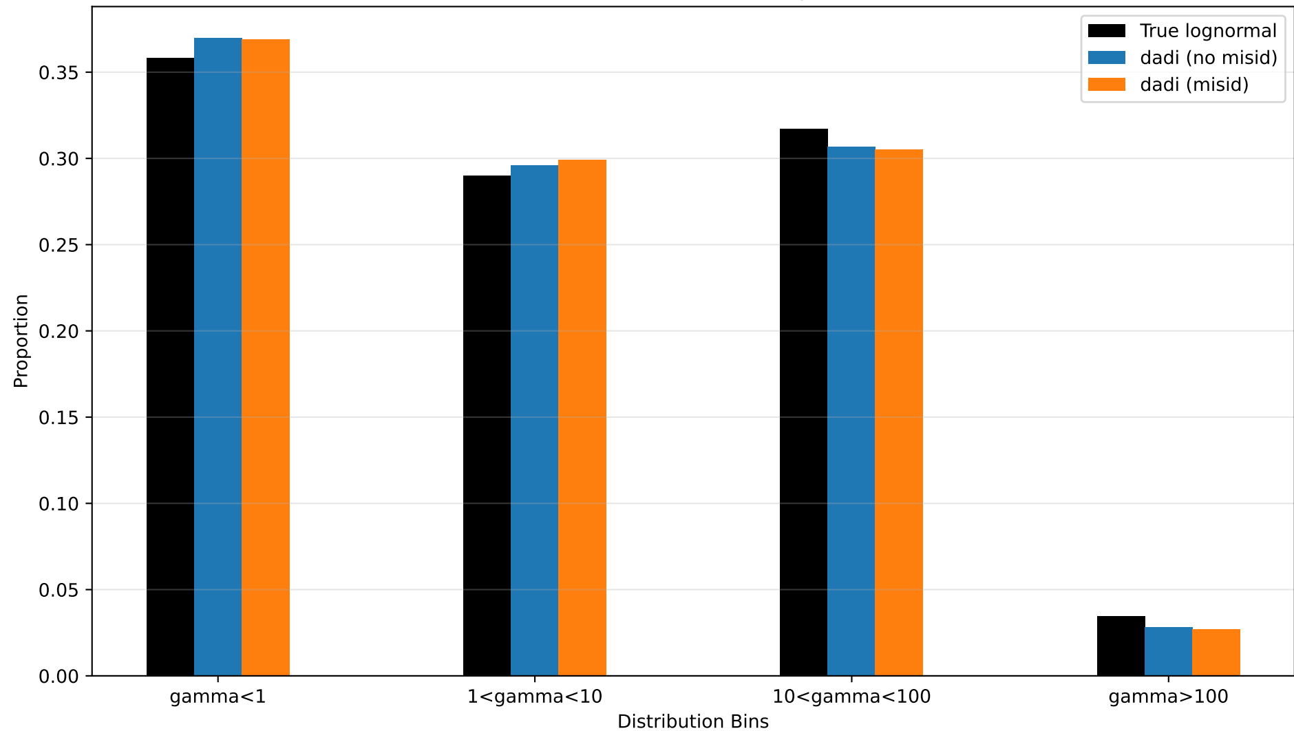
Discretized DFE Distribution Comparison: small
