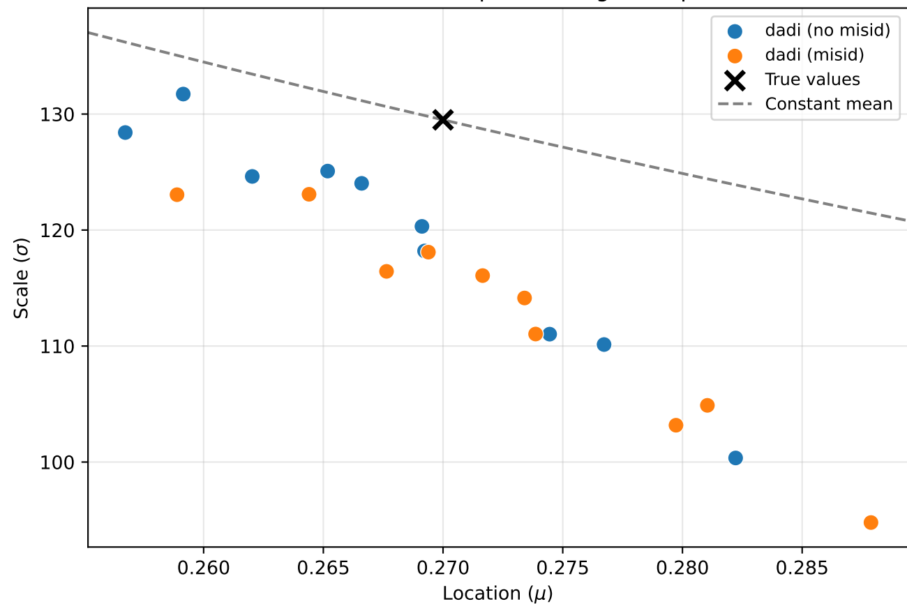
DFE Inference Allotetraploids (Large Sample Size)
