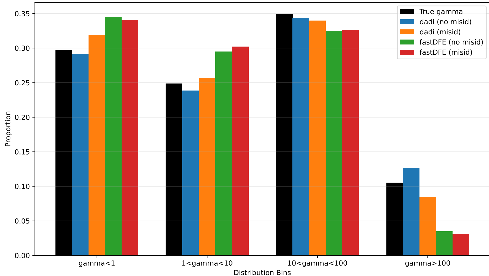
Discretized DFE Distribution Comparison: large
