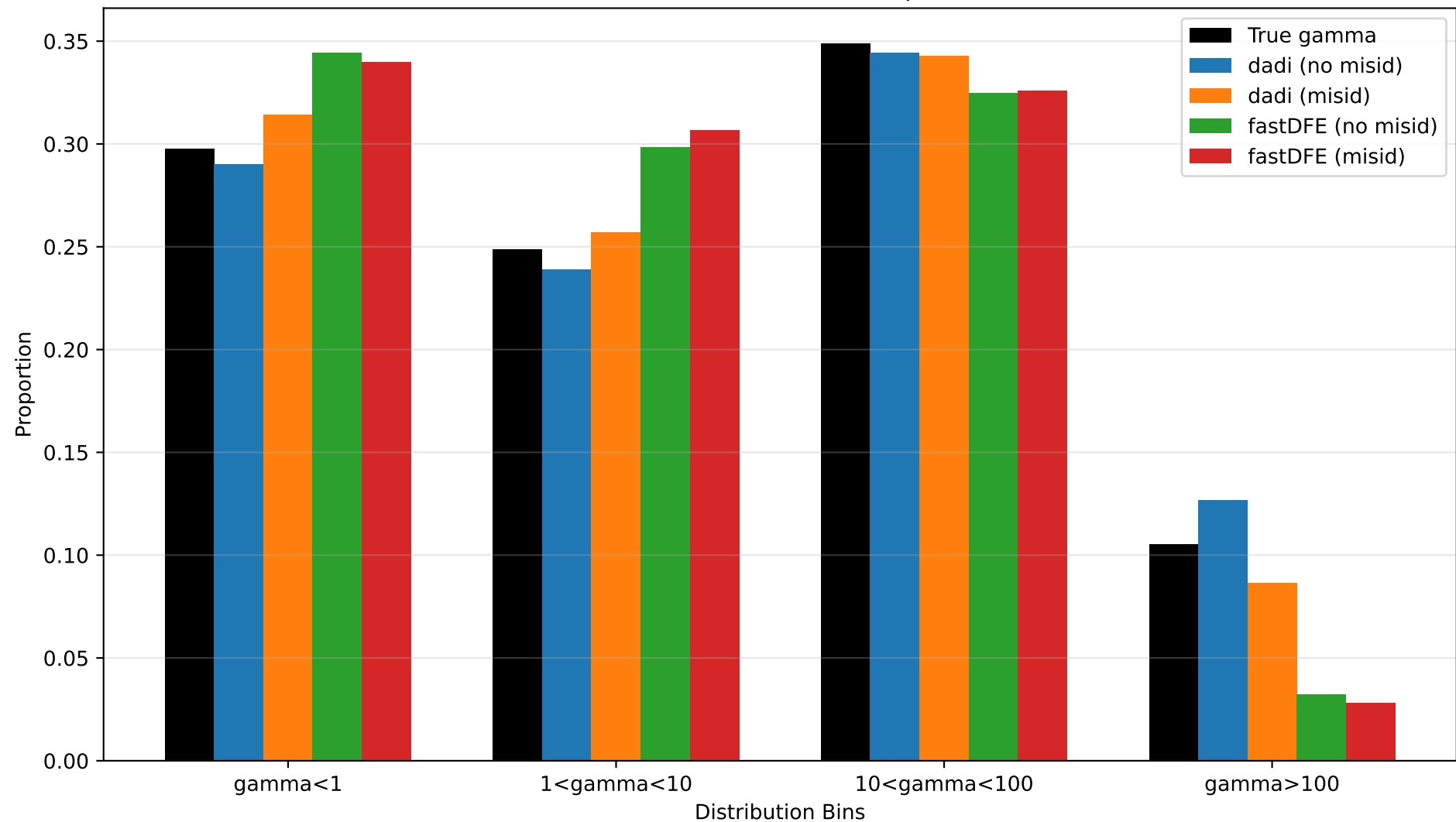
Discretized DFE Distribution Comparison: med
