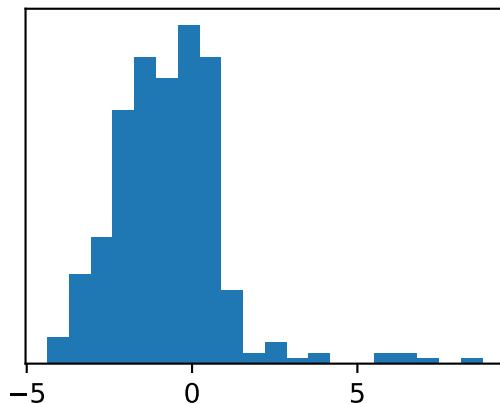
residuals
