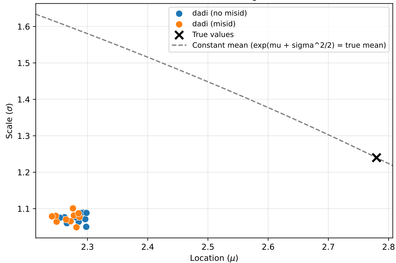
DFE Inference: large
