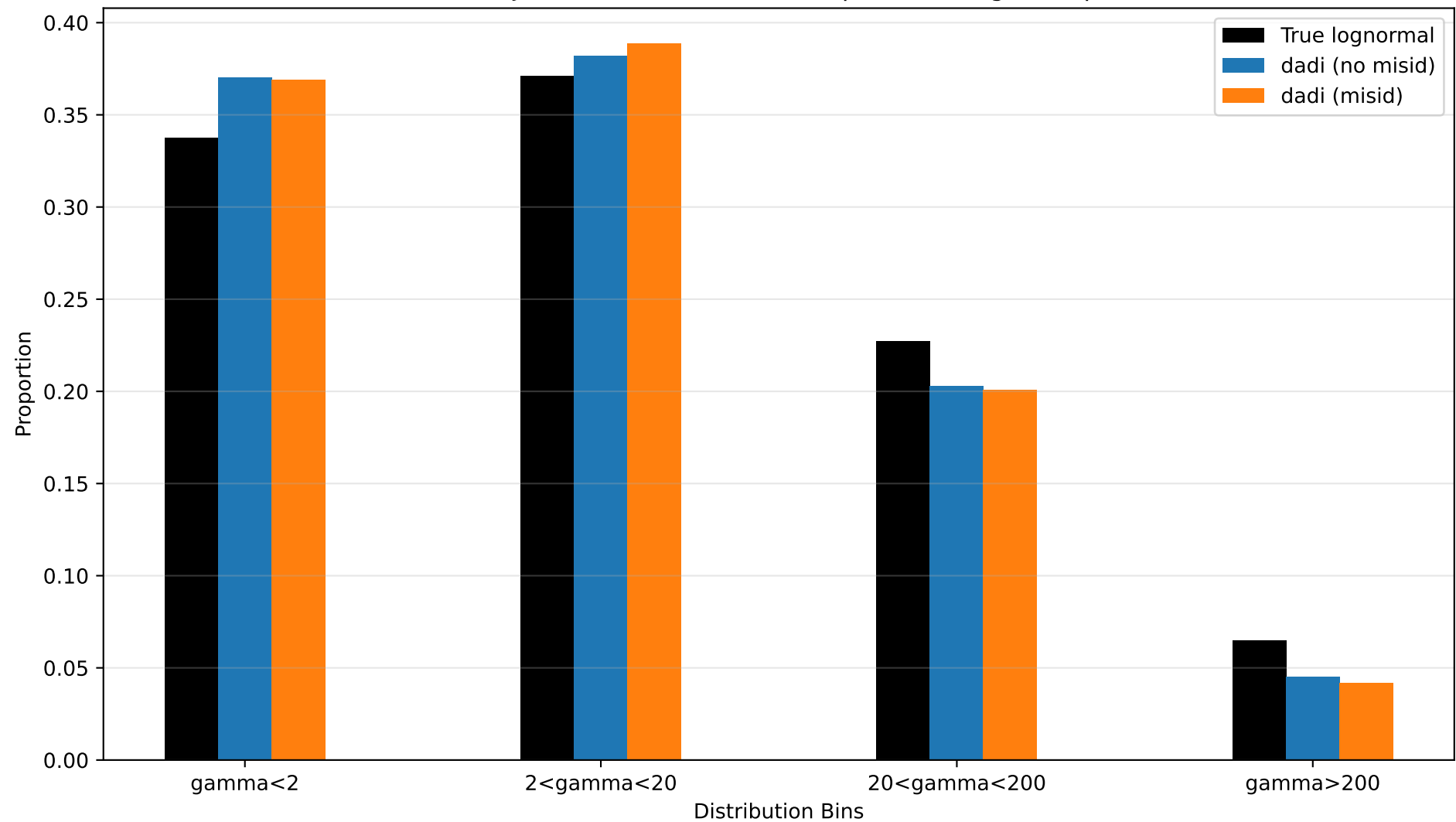
Discretized Joint DFE Distribution Comparison (Large Sample Size)
