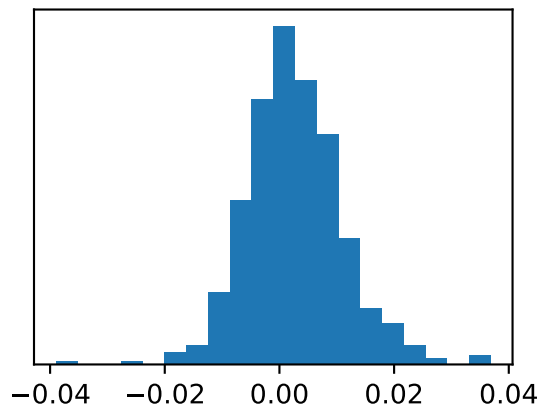
residuals
