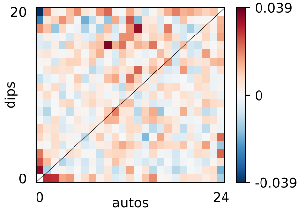
residuals
