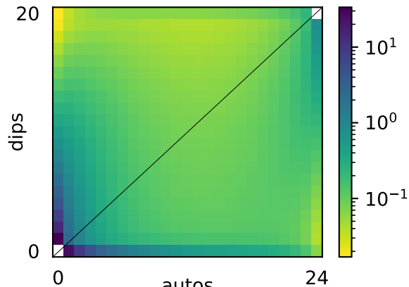
residuals
