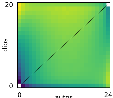
residuals
