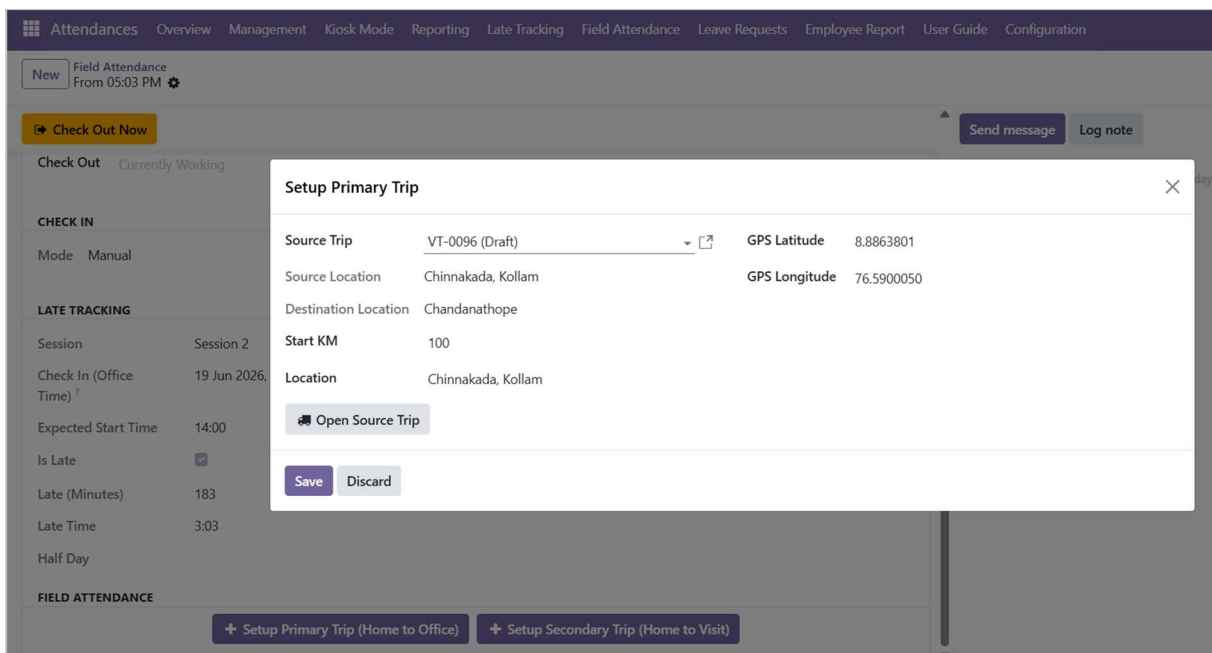
Setup Primary Trip — pick a trip, enter Start KM and save.
