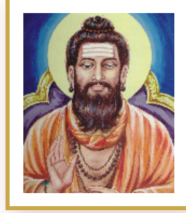
Allamaprabhu
