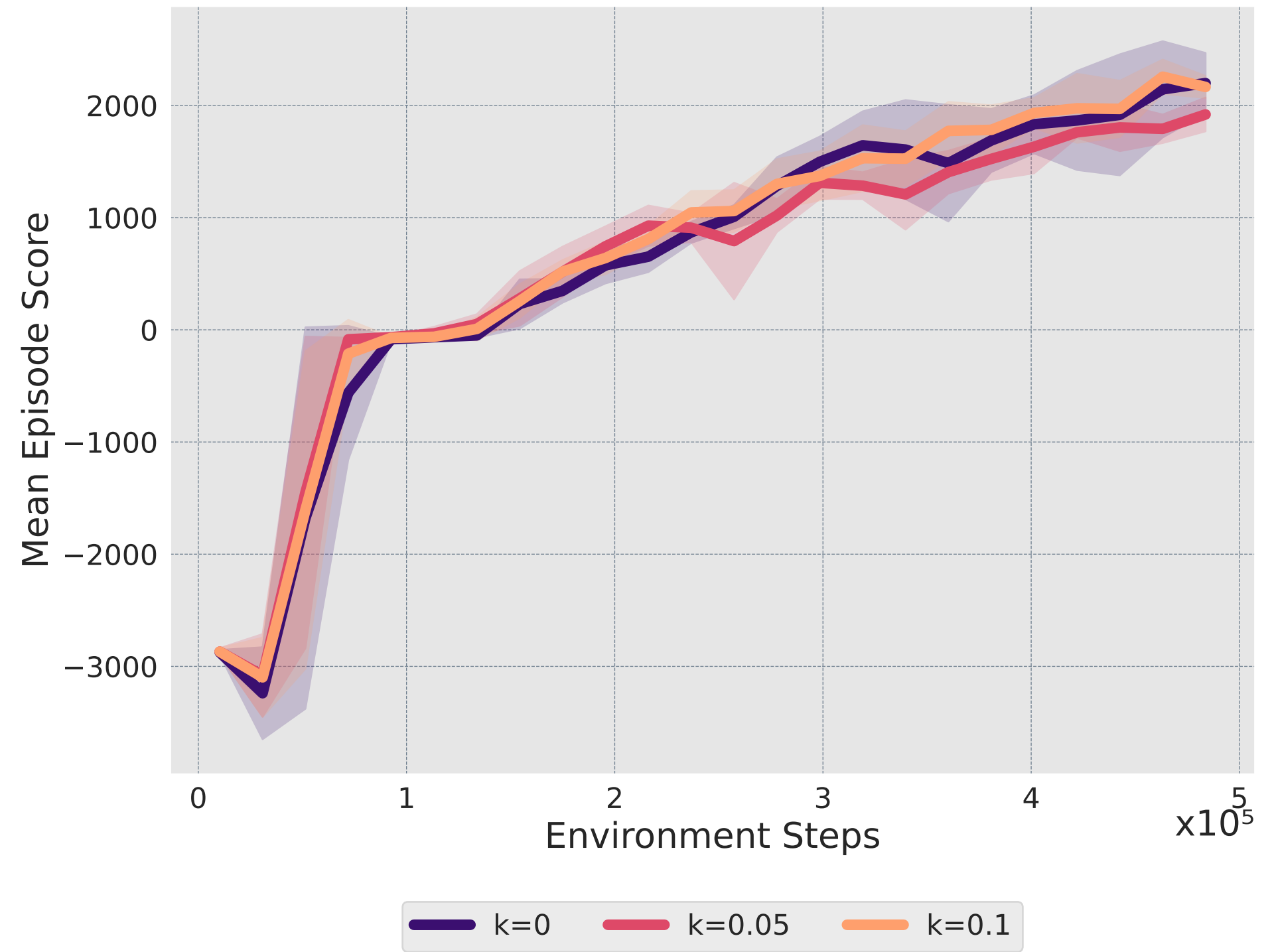
HalfCheetah-v5 (Control Cost - 10x)
