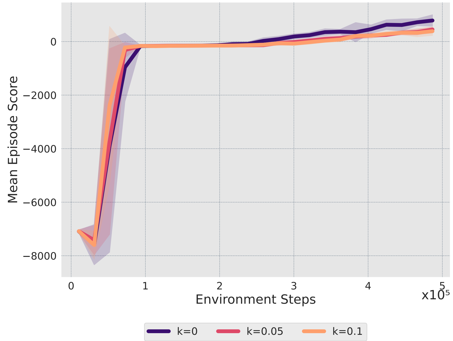
HalfCheetah-v5 (Control Cost - 25x)
