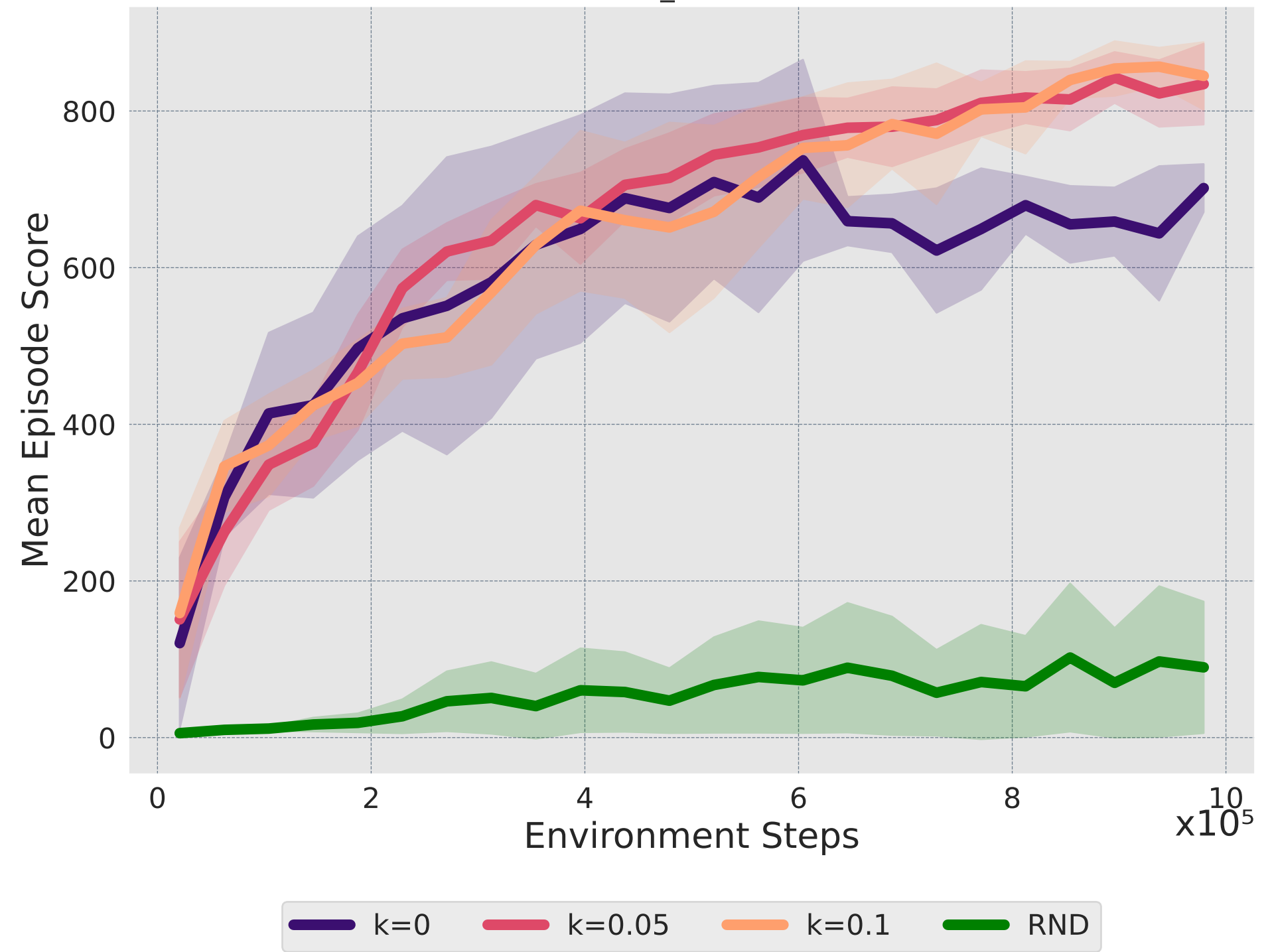
cheetah_run (Vision)
