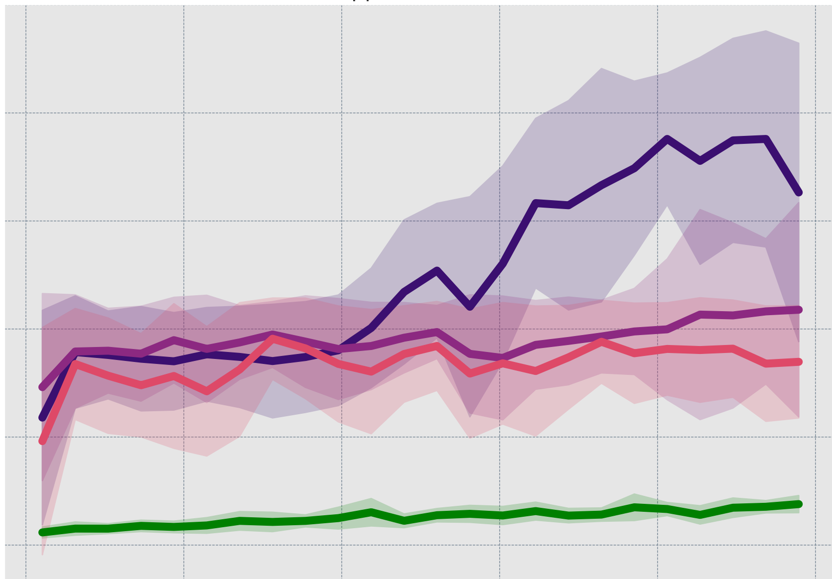
Hopper-v5 (Vision)
