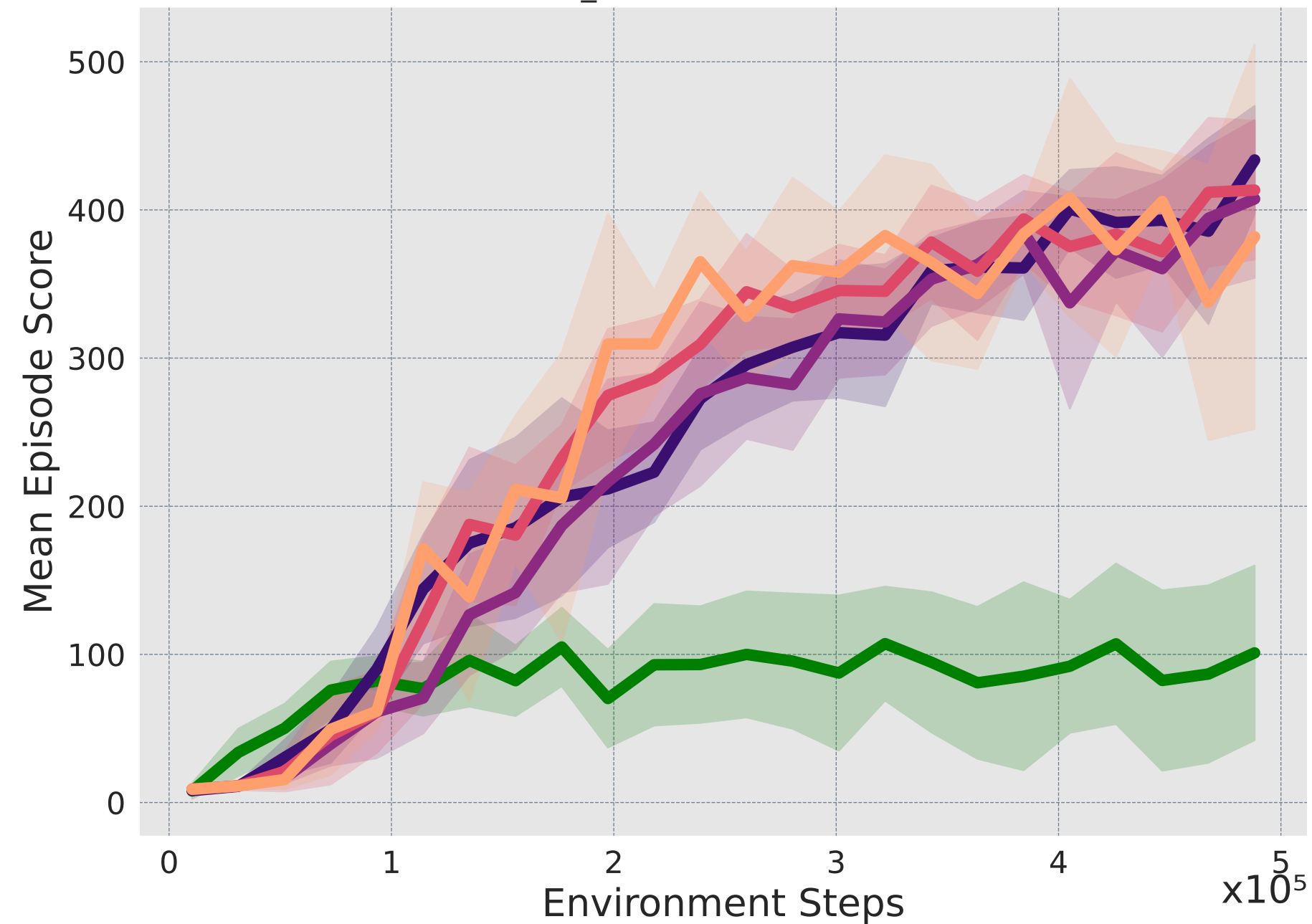
cheetah_run (Partial Observations)
