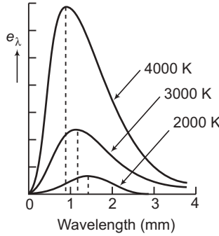
Power of black body radiation versus wavelength at three temperatures. Note that the amount of radiation emitted (the area under a curve) increase with increasing temperature.
